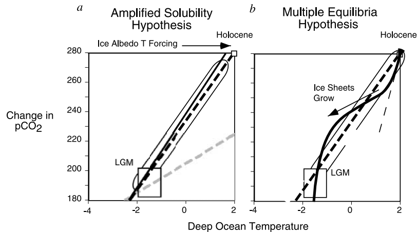
Figure 6. Schematic of the alternative scenarios for the interplay between the solubility and the radiative CO 2 relations during the LGM. The oval outlines the relation between CO 2 and temperature indicated by the paleodata. (a) Aspects of the climate system linked to temperature change, such as deep water formation and sea ice, could lead to larger changes in CO 2 effectively enhancing solubility. The gray dashed line is the solubility relation as shown in Figure 1. The combined effect of solubility and other mechanisms linked to temperature forcing shown by the black dashed line is the enhanced solubility relation. The enhanced solubility relation is steeper than the model derived solubility (gray dashed line) and nearly overlaps with the radiative relation (solid line, the same relation described in Figure 1). The similar slopes of the two relations would result in amplified feedback between CO 2 and temperature, making the system very sensitive to small perturbations. (b) Combining the effect of nonlinear ice albedo feedback with the radiative feedback would result in a system with multiple equilibria. The radiative relation is shown by the solid black curve. At CO 2 and ice volume near Holocene conditions, the relation is identical to the modeled radiative effect of for the CO 2 -only scenario as shown in Figure 5; this is also shown by the thin dashed line. As temperature approaches freezing, further decreases in CO 2 cannot greatly reduce temperature thus there is a slope similar to the radiative relation at high CO 2 /low ice volume. Connecting these extremes yields the radiative relation associated with large changes in ice volume. We use the enhanced solubility relation from Figure 6a (the thick gray dashed line). Intersections between the two relations define multiple equilibria.
