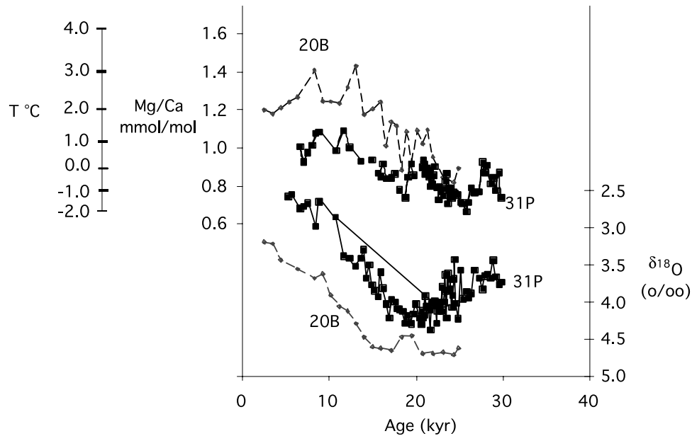
Figure 2. Mg/Ca, Mg-derived temperatures, and \delta^{18}\text{O} in cores TR163-31P and TR163-20B. The black solid lines and squares represent data from core TR163-31P. The gray dashed lines and triangles represent data from core TR163-20B. Temperature estimates are derived using the empirically derived equation for Uvigerina sp.: \text{Mg/Ca} = 0.87\exp(0.15 \cdot T) . Data from TR163-31P were previously published in the work of Martin et al. [2002b].
