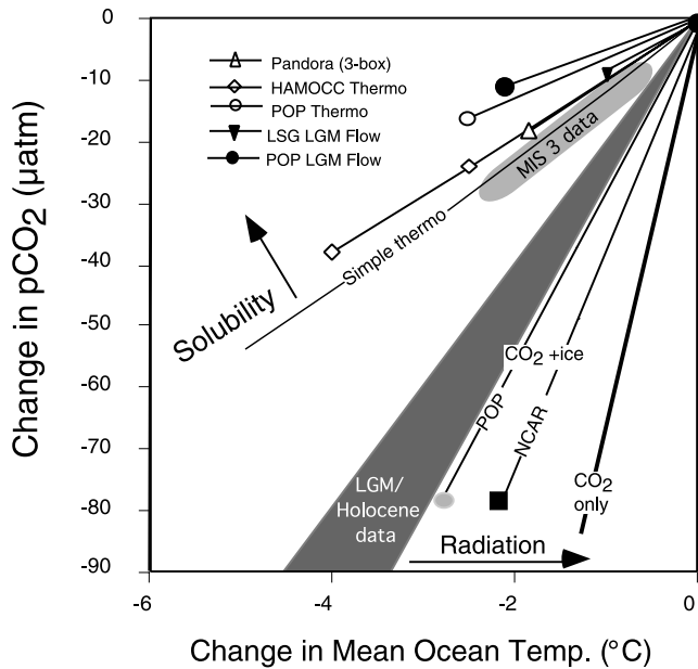
Figure 5. Model relationships between deep ocean temperature and the pCO 2 of the atmosphere. Solid line (“simple thermo”) is the solubility of CO 2 gas into a homogeneous seawater solution, decreasing from 278 µatm. Pandora, HAMOCC Thermo, and POP (Los Alamos National Laboratory’s Parallel Ocean Program) Thermo are new numerical experiments using global circulation carbon cycle models of the ocean, showing the effects of changing the solubility of the CO 2 gas only, with no changes in circulation or mixing of the ocean. LSG LGM and POP LGM are GCM results of changing the sea surface temperature forcing at the sea surface, which changes both CO 2 solubility and ocean circulation. These are all estimates of the solubility relation between CO 2 and deep sea temperature. “CO 2 only” is from the GFDL coupled climate model equilibrium run of doubled CO 2 described by Stouffer and Manabe [Stouffer and Manabe, 1999]. NCAR Greenhouse is from the NCAR CCSM coupled climate model runs described by Shin et al. [2003]. POP Greenhouse is the result of driving the POP ocean model using sea surface forcing from the Shin et al. [2003] simulation. These are both estimates of the radiative relation between CO 2 and deep sea temperature with CO 2 specified. Gray regions are estimates of the CO 2 /deep ocean T relation derived from paleodata for stage 3 and for the deglaciation.
