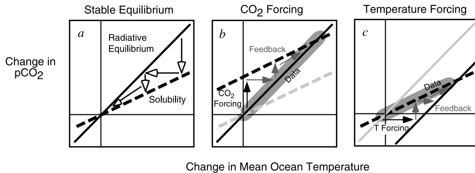
Figure 1. Schematic of the interplay between the solubility and the radiative CO 2 relations. (a) Solubility relation (dashed line) and radiative relation (solid line). The CO 2 concentration tends to relax vertically toward the solubility relation when forced by changing T, whereas T, forced radiatively by CO 2 , relaxes horizontally toward the radiative line. Coupled together, the system relaxes toward the intersection of the two relations (open-headed arrows). (b) Effect of CO 2 forcing, such as changing the biological pump or the pH of the ocean. As the system relaxes to the new intersection between solubility and radiative relations, the original CO 2 forcing is amplified. Paleo-CO 2 and deep ocean temperature data would covary along the radiative relation (gray stippled region). (c) Effect of forcing the deep sea temperature, as by changing the circulation in the North Atlantic. The original temperature forcing is amplified by the changing solubility of CO 2 . Paleodata would fall along the solubility relation (stippled region).
